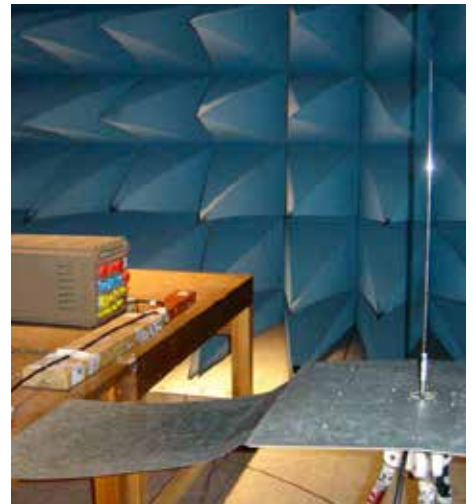
THE CM-ATR-45/SIXHEX PASSES ELECTROMAGNETIC EMISSION & RADIATION TEST. RADIATED E FIELD 2 MHz to 30 MHz. MIL-STD-461E CERTIFICATE AVAILABLE.
